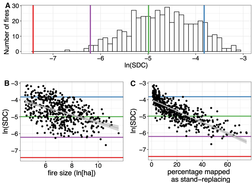
Fig. 5 Distribution of the natural logarithm of the stand-replacing decay coefficient ( \ln(\text{SDC}) ) estimated for 477 fires in California between 1984 and 2015 (a). Plots of SDC as a function of the log of the fire size (b) and percent stand-replacing (c) are also shown. The four colored lines correspond to the colors and patch configurations in Fig. 2. Smaller values of \ln(\text{SDC}) indicate fires with much of their stand-replacing area far from the patch edge
