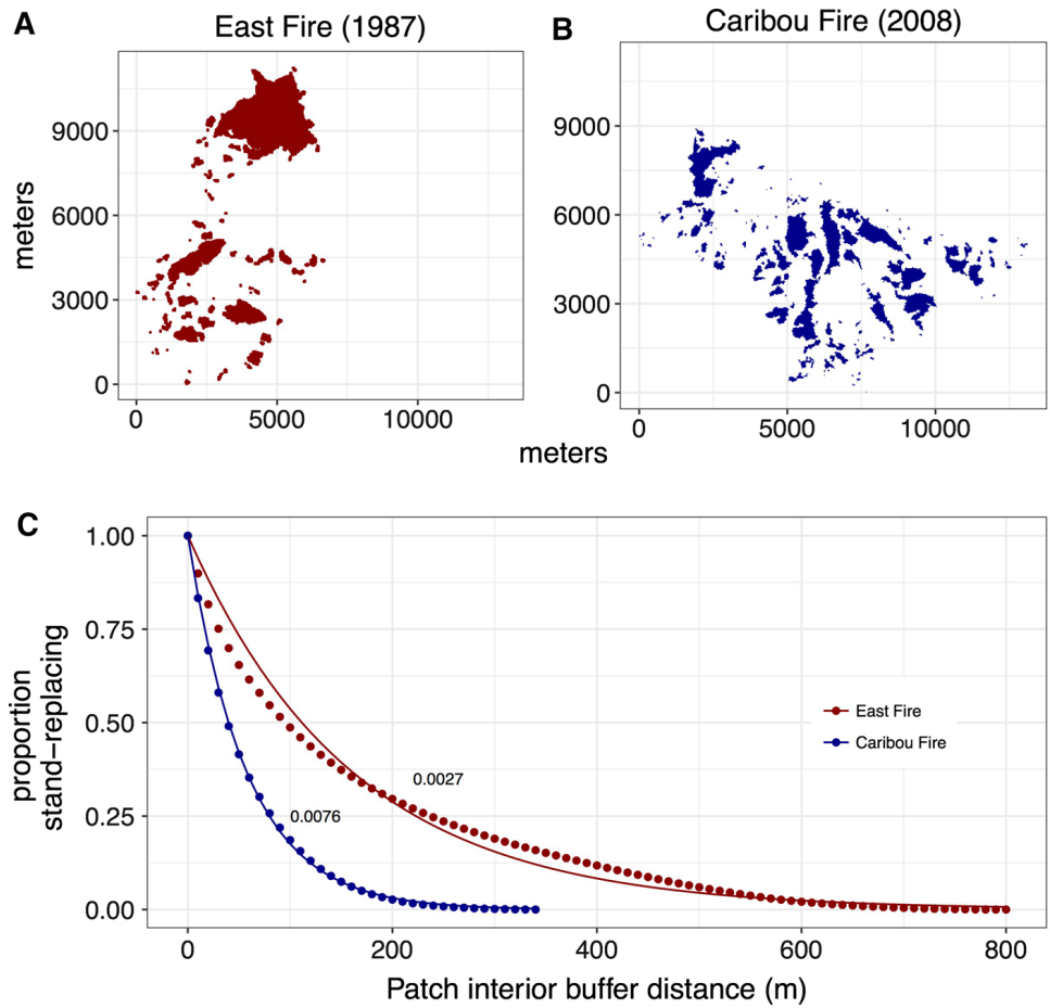
Fig. 4 Stand-replacing area for two example wildfires that occurred in the Klamath region, northwestern California, USA (a, b). Both fires have similar total area (4643 and 5319 ha) and stand-replacing proportions (20%), but different spatial distribution of stand-replacing area. These different patterns are captured by the plots showing how stand-replacing area is distributed as a function of interior buffer distance (c). Points indicate observed proportions for a given distance, while solid lines are the proportions predicted by Eq. 1 fit to the point data. The stand-replacing decay coefficient (SDC) is reported for each fire
